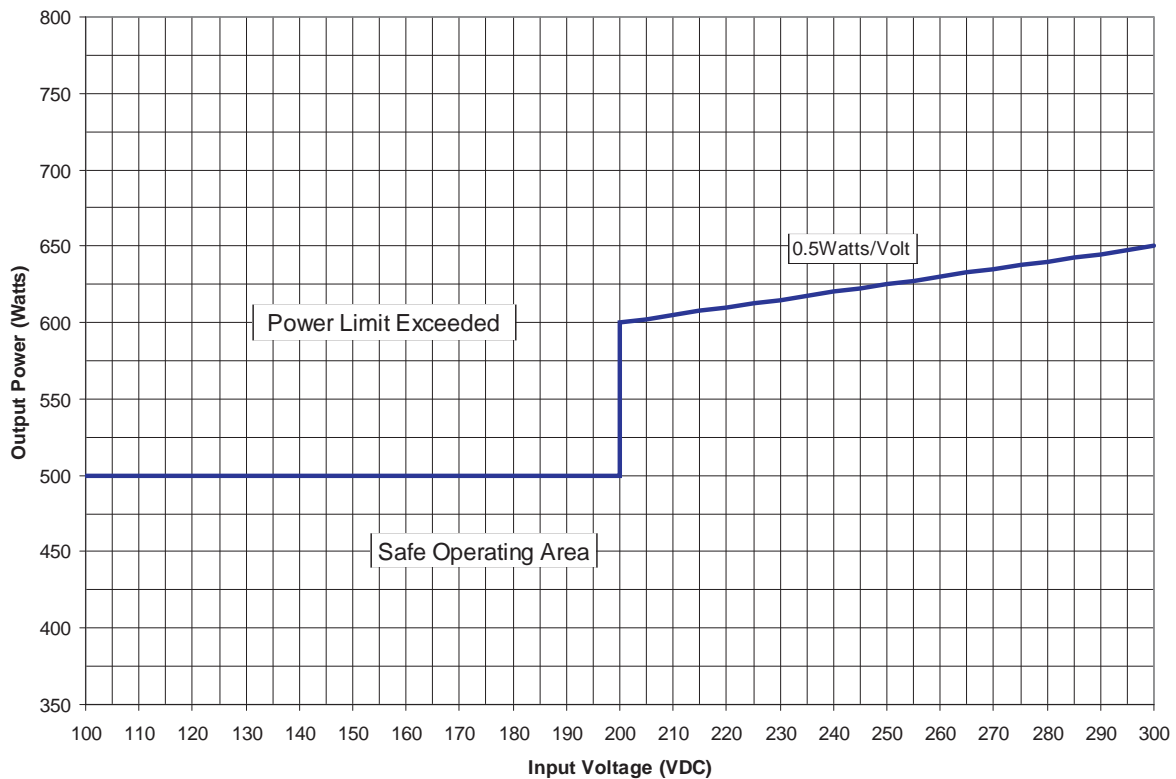
PFC Micro Output Power vs. DC Input Voltage
