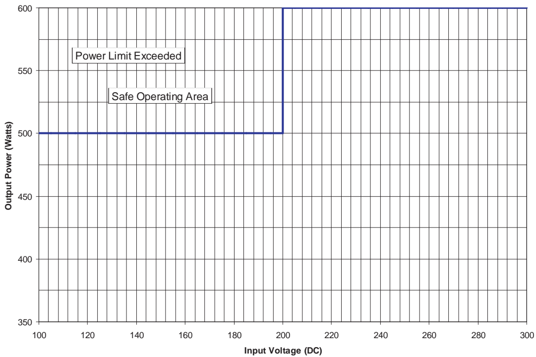
PFC MicroS Output Power vs. DC Input Voltage
