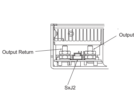
Figure 3. Power Connections for Single Output
