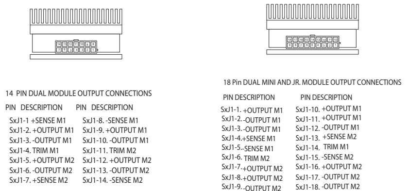
Figure 4. Power connections for Dual Output
